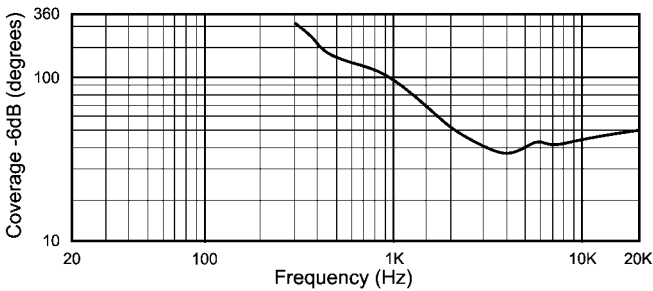
Vertical coverage
