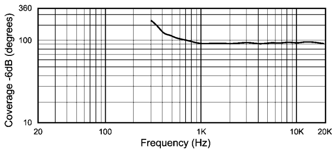
Horizontal coverage
